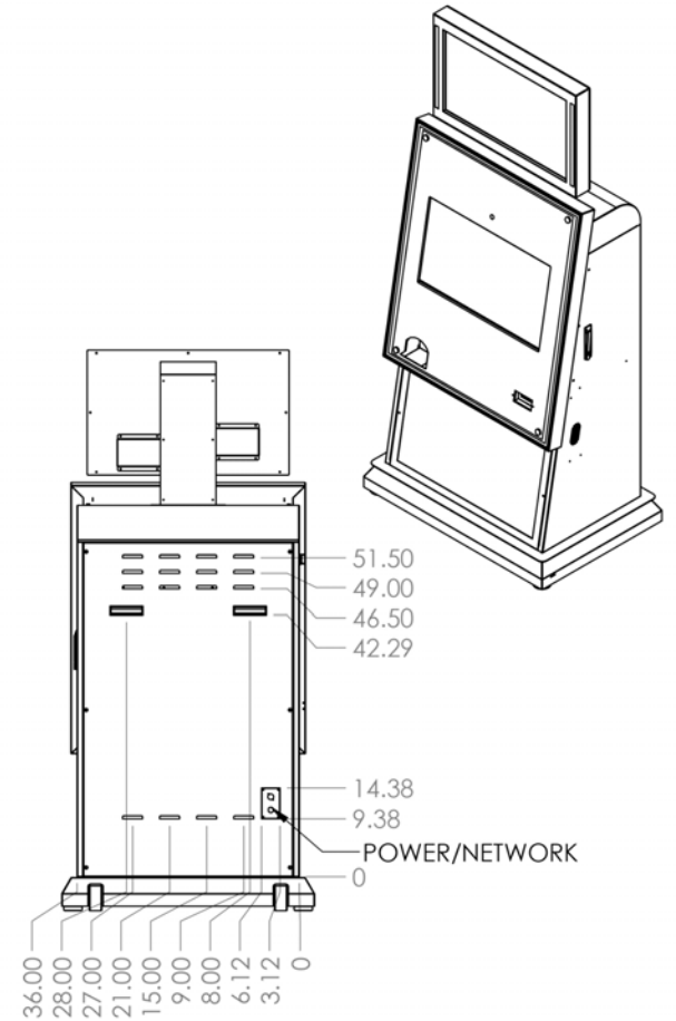
SeePoint Business Kiosk Systems TITLE: CARD PRINTING KIOSK GENERAL DIMENSIONS
